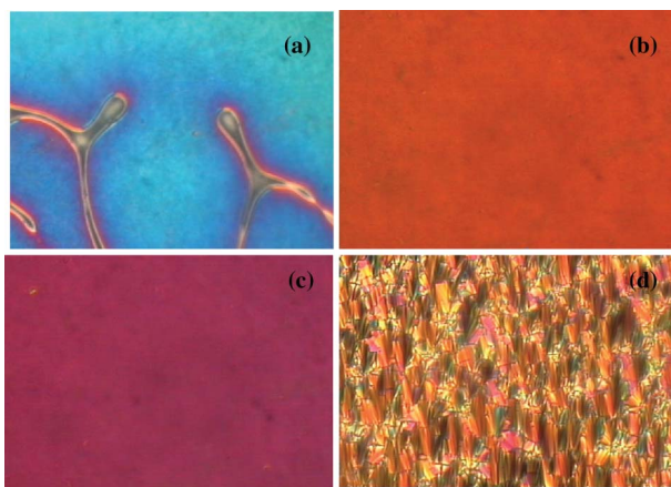
Figure 10. Representative textures of Mix3 at different temperatures: in the N phase at: (a) 63°C; (b) 50.6°C; (c) 40°C; and (d) in the SmC phase at 26°C. Pictures cover an area of 0.4 mm \times 0.3 mm.
